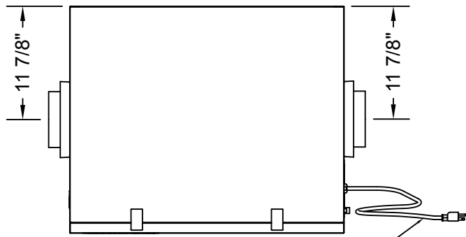
34" Line Cord TOP VIEW
