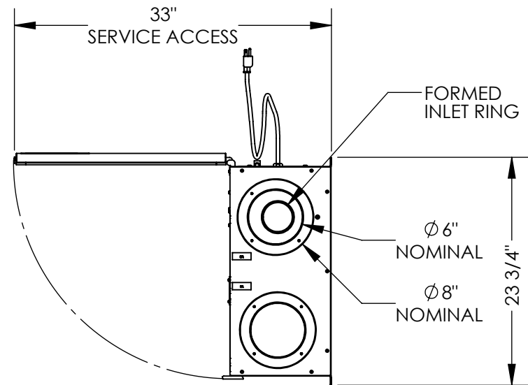
RIGHT VIEW
