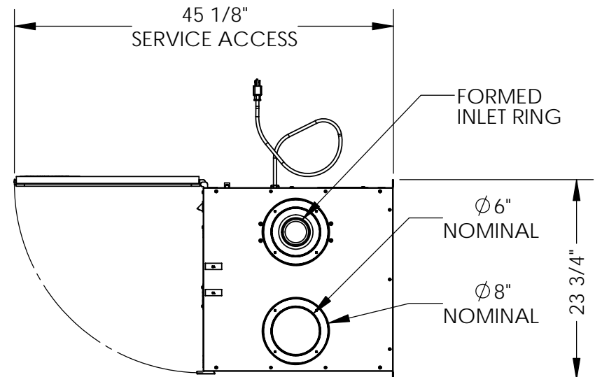
RIGHT VIEW
