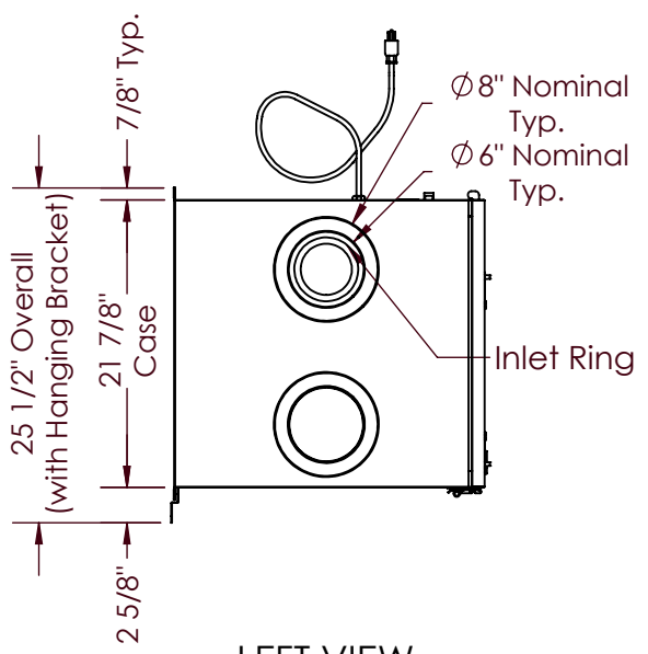
LEFT VIEW
